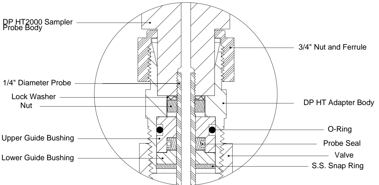
Section View - Hot Tap Adapter
